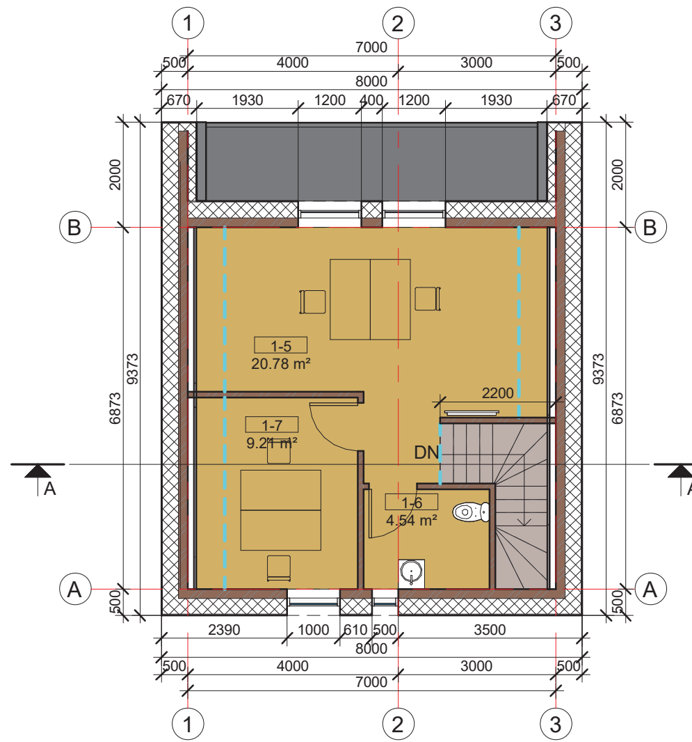
MANSARDOS PLANAS M1:100
